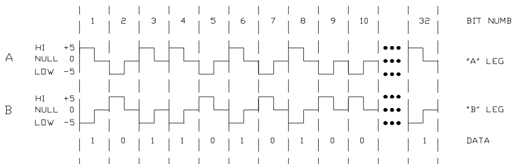
Figure 1. ARINC 429 Bit Encoding Example
